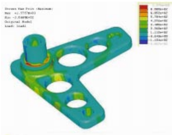
Typical Pro/Mechanica Stress plot
